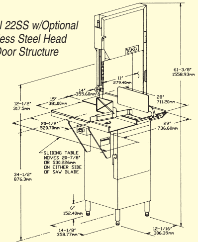
Model 22SS Trim Saw available w/optional Stainless Steel Head and Door Structure and Front Stationary Table
