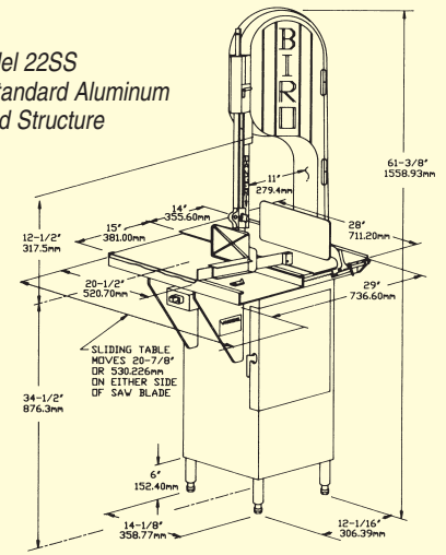
Model 22SS w/Optional Stainless Steel Head and Door Structure
